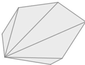
Figure 1.7: A convex polygon divided into triangles.
